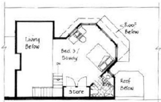
First Floor (Mezzanine) Plan 1:100
